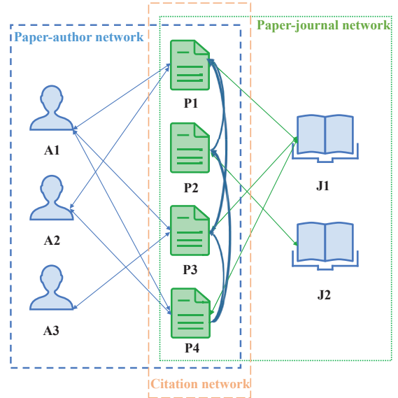
Figure 1: Illustration of heterogeneous academic networks.
