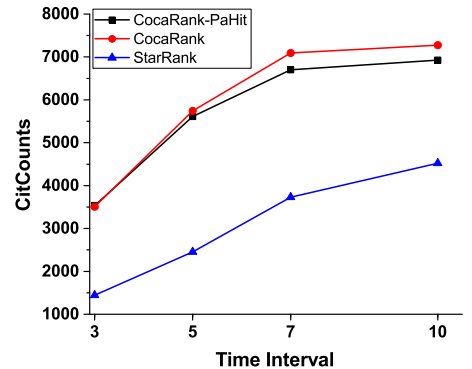
Figure 2: Comparison of future average CitCounts in different time intervals.
